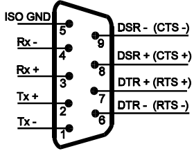
RS 422 side
